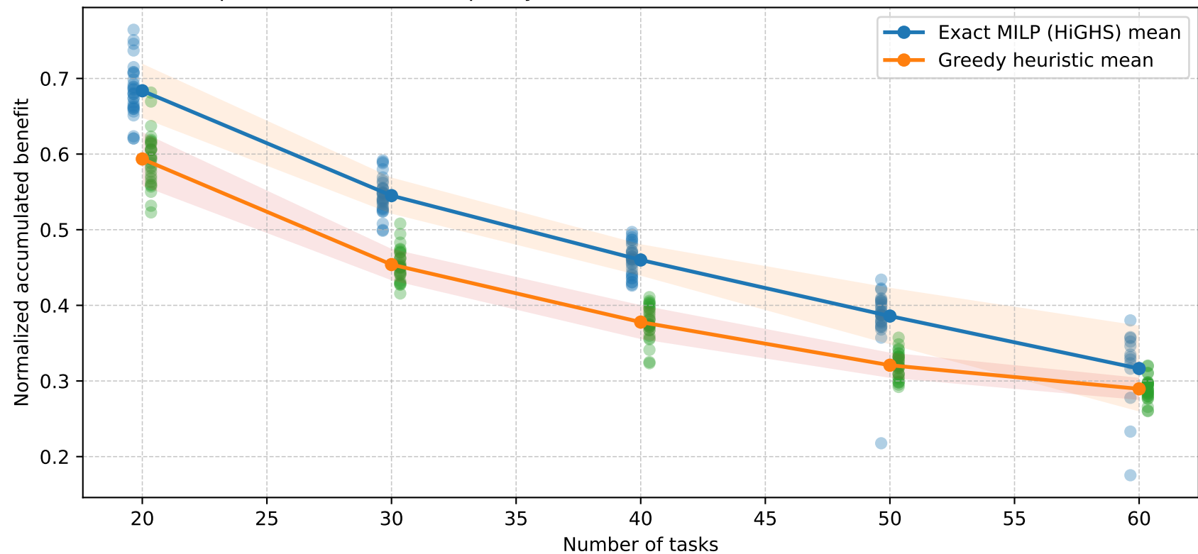
Experiment B: Solution quality across scaled TTAP instances - 6 Helos / 7 Areas
